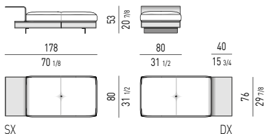
PANCA CON FLAP CM 178X80 BENCH WITH FLAP CM 178X80
