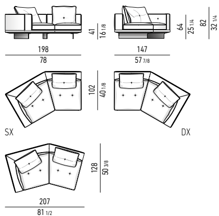
ELEMENTO TERMINALE INCLINATO CM 198X147 INCLINED ELEMENT WITH ARMREST CM 198X147
